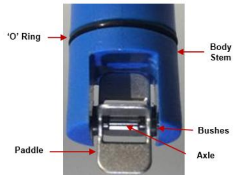
Paddlewheel Sensor
