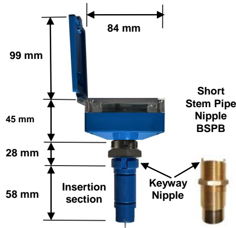
Standard 'Short Stem' body version, pipe ID up to 100mm ID Side view dimensions
