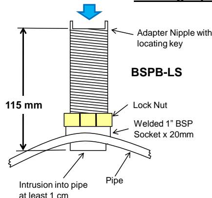
Fig. 1 Installing Into Existing Pipeline
