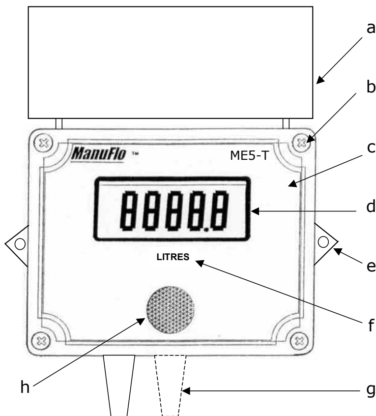
Figure 1. External view of ME5-T Totaliser Indicator
